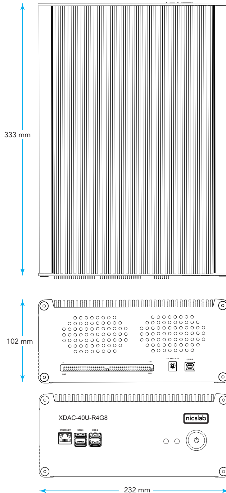
Figure 2. Product Dimension
