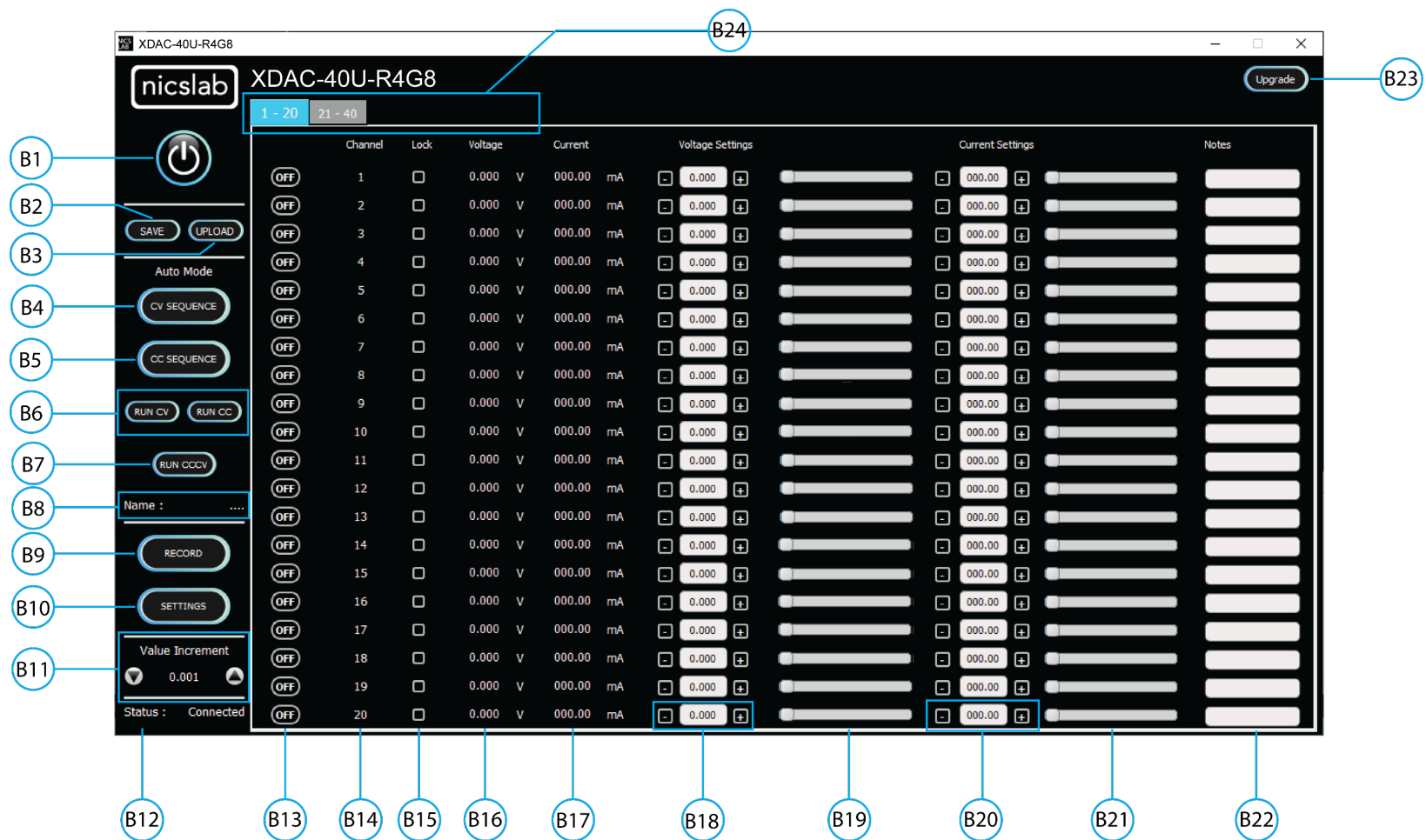
Figure 4. GUI
