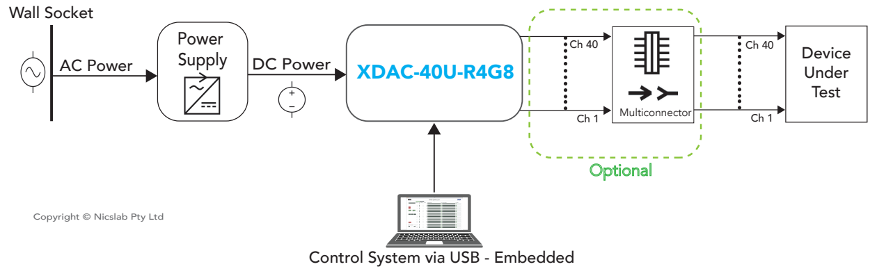
Figure 1. XDAC-40U-R4G8 System Diagram
